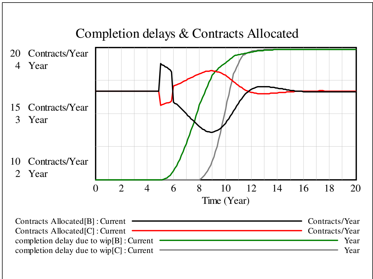
Example Simulation output -- contractors model
